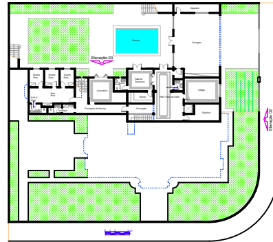
Subsolo A = 338,18 m 2
